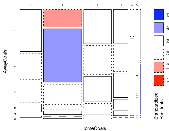
Figure 2: Friendly mosaic plot for the Bundesliga data.
